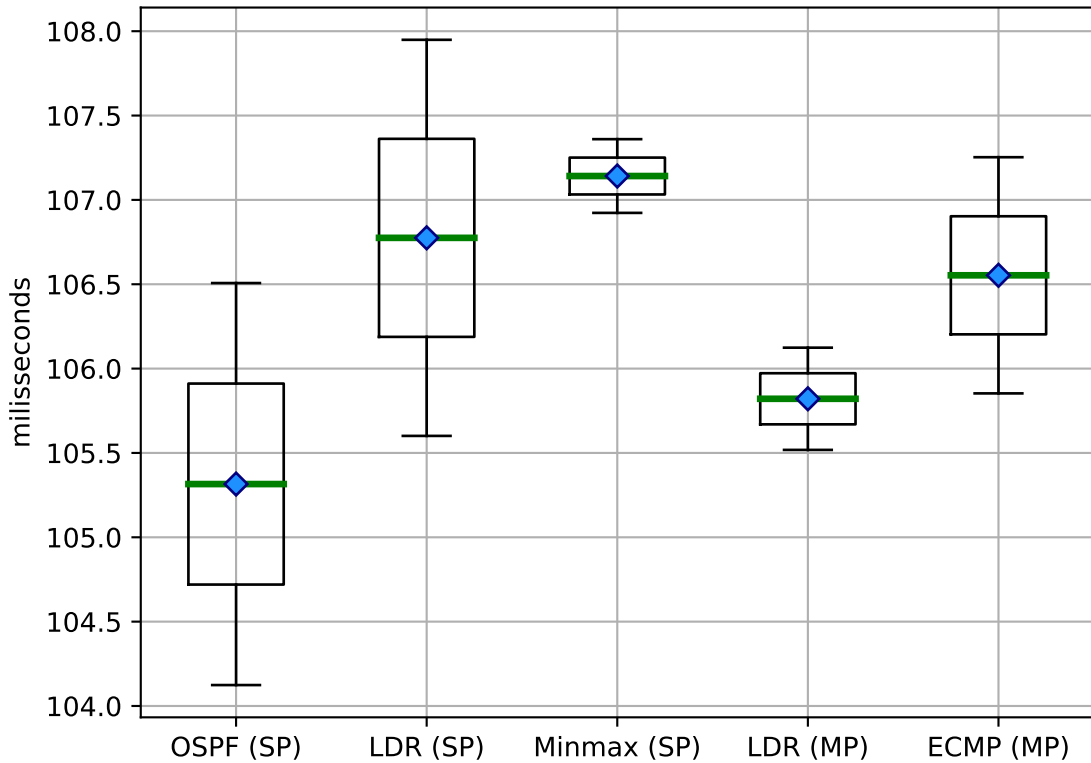
Jitter (concurrent) on Binary Tree
