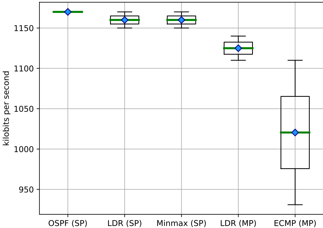
Bandwidth (sequential) on Triangle
