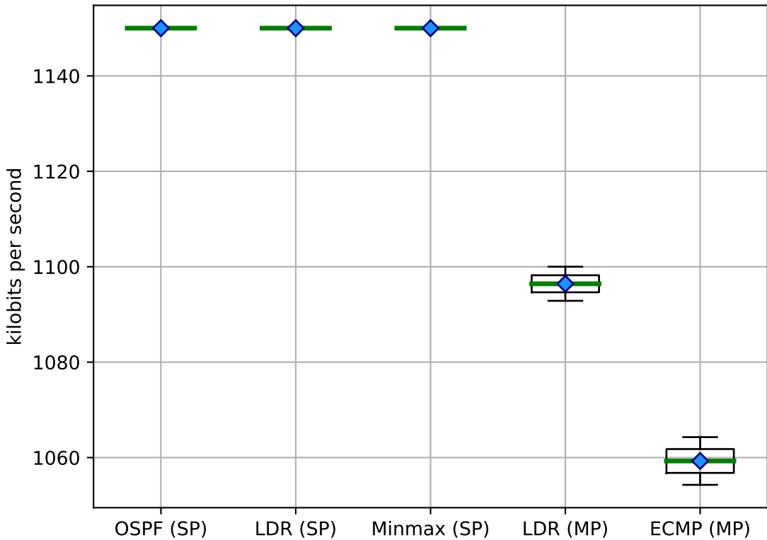
Bandwidth (sequential) on Grid
