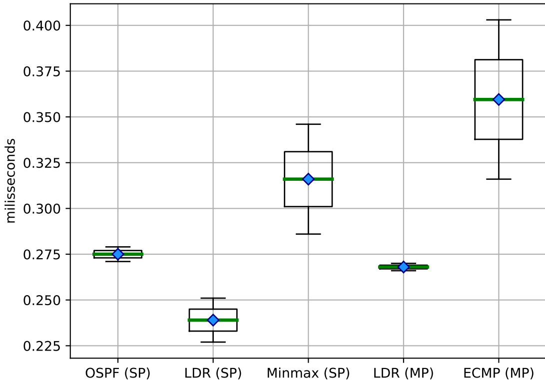
Jitter (sequential) on Fat Tree
