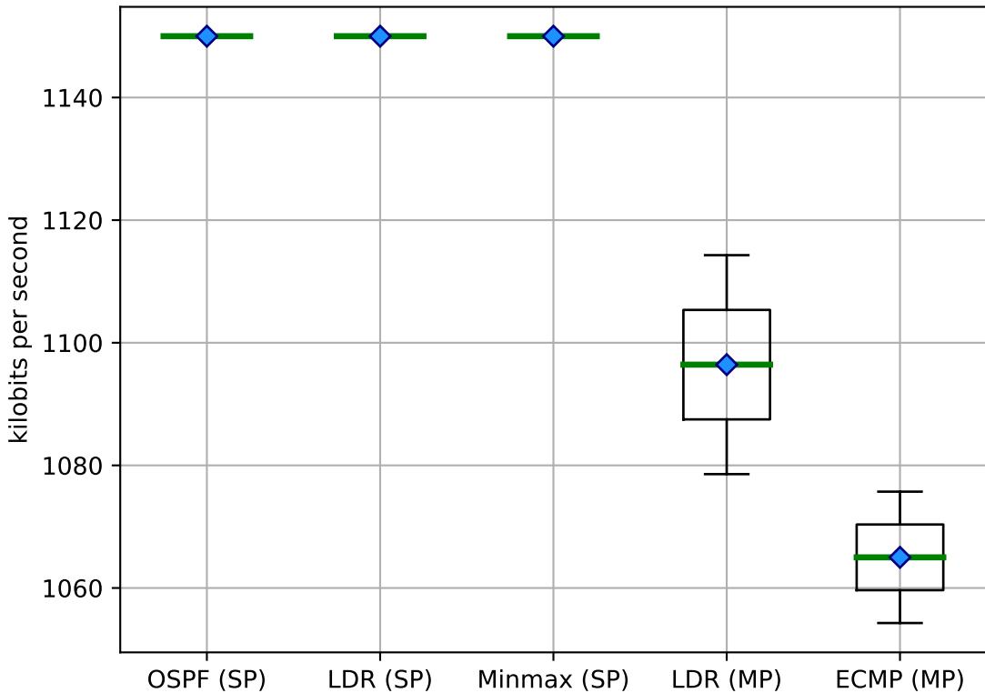
Bandwidth (sequential) on Fat Tree
