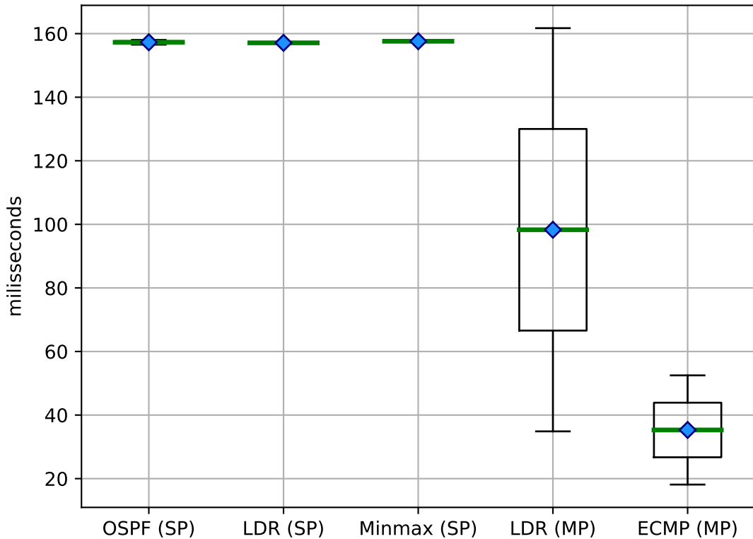
Latency (concurrent) on Fat Tree
