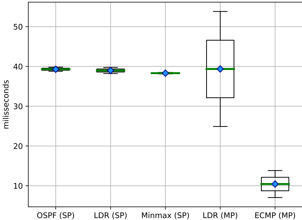
Jitter (concurrent) on Fat Tree
