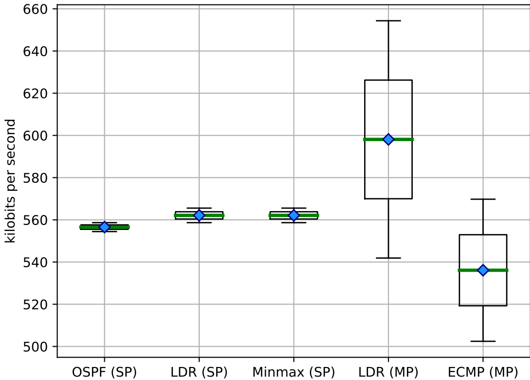
Bandwidth (concurrent) on D-Cell
