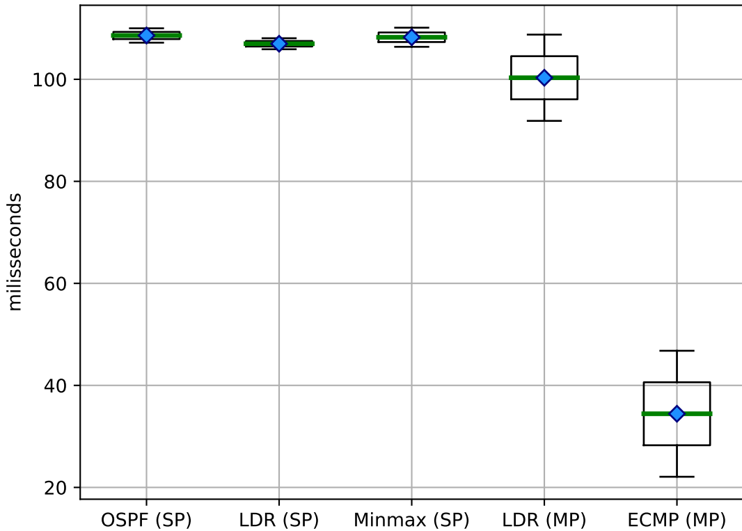
Jitter (concurrent) on 5-layered CLOS
