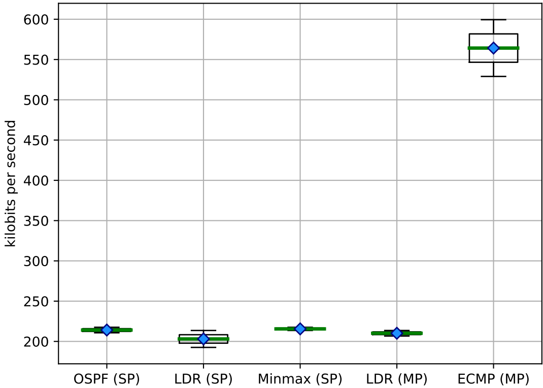
Bandwidth (concurrent) on 5-layered CLOS
