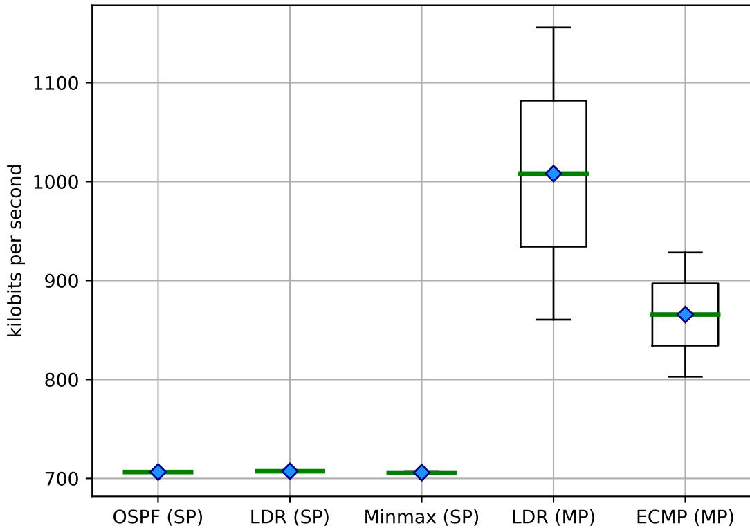
Bandwidth (concurrent) on 3-layered CLOS
