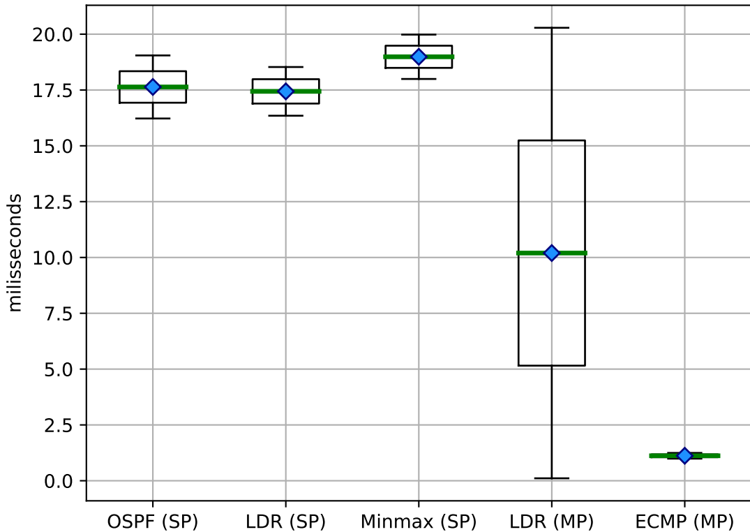
Latency (concurrent) on B-Cube
