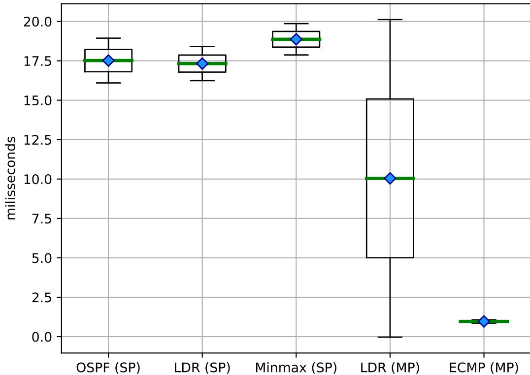
Latency (impact) on B-Cube
