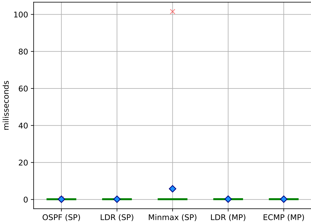
Latency (sequential) on All
