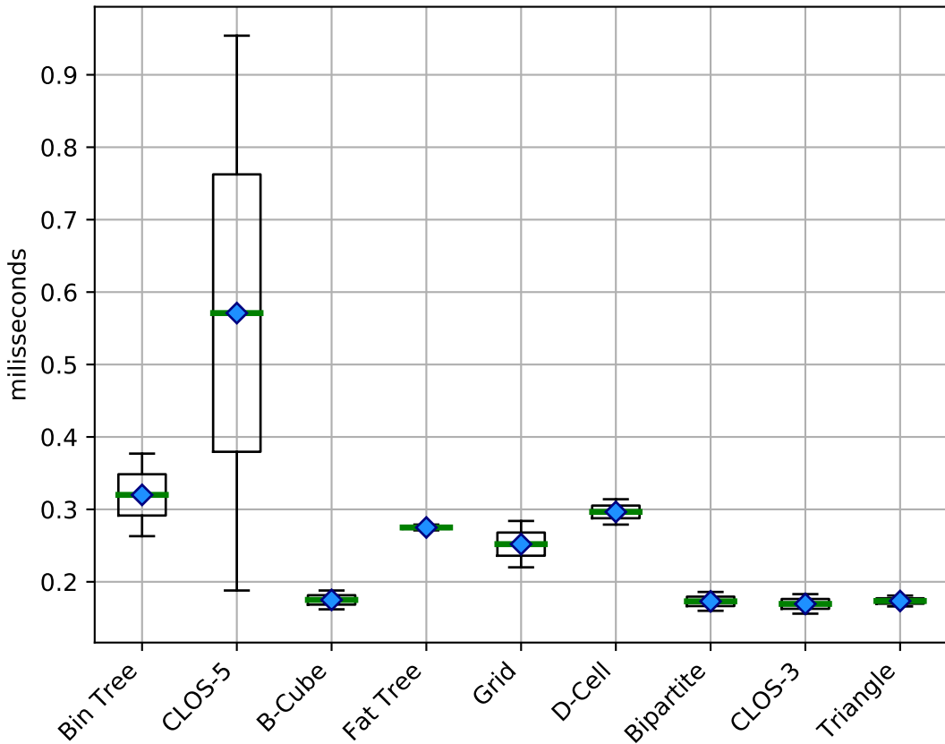
Jitter (sequential) using OSPF (single-path)
