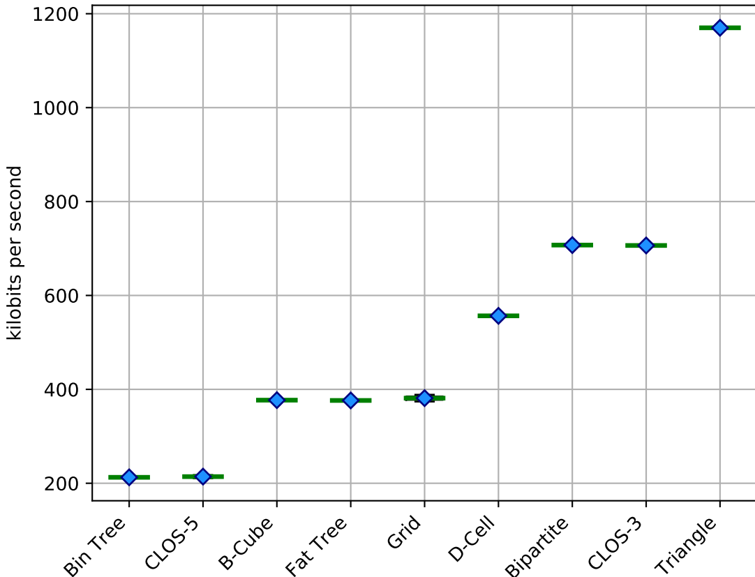
Bandwidth (concurrent) using OSPF (single-path)
