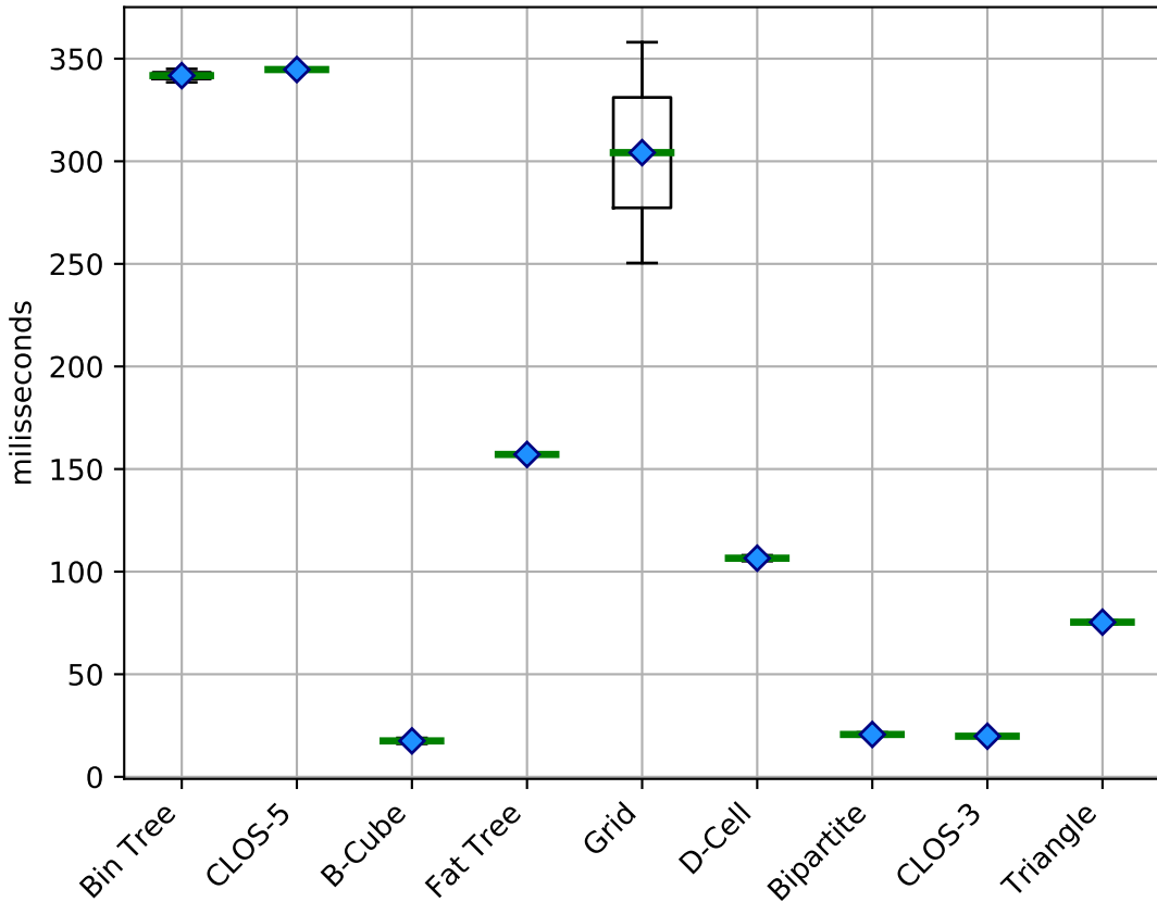
Latency (impact) using OSPF (single-path)
