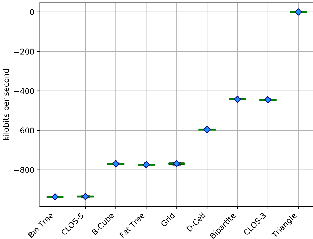
Bandwidth (impact) using OSPF (single-path)
