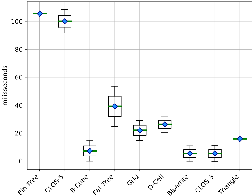
Jitter (impact) using LDR (multi-path)
