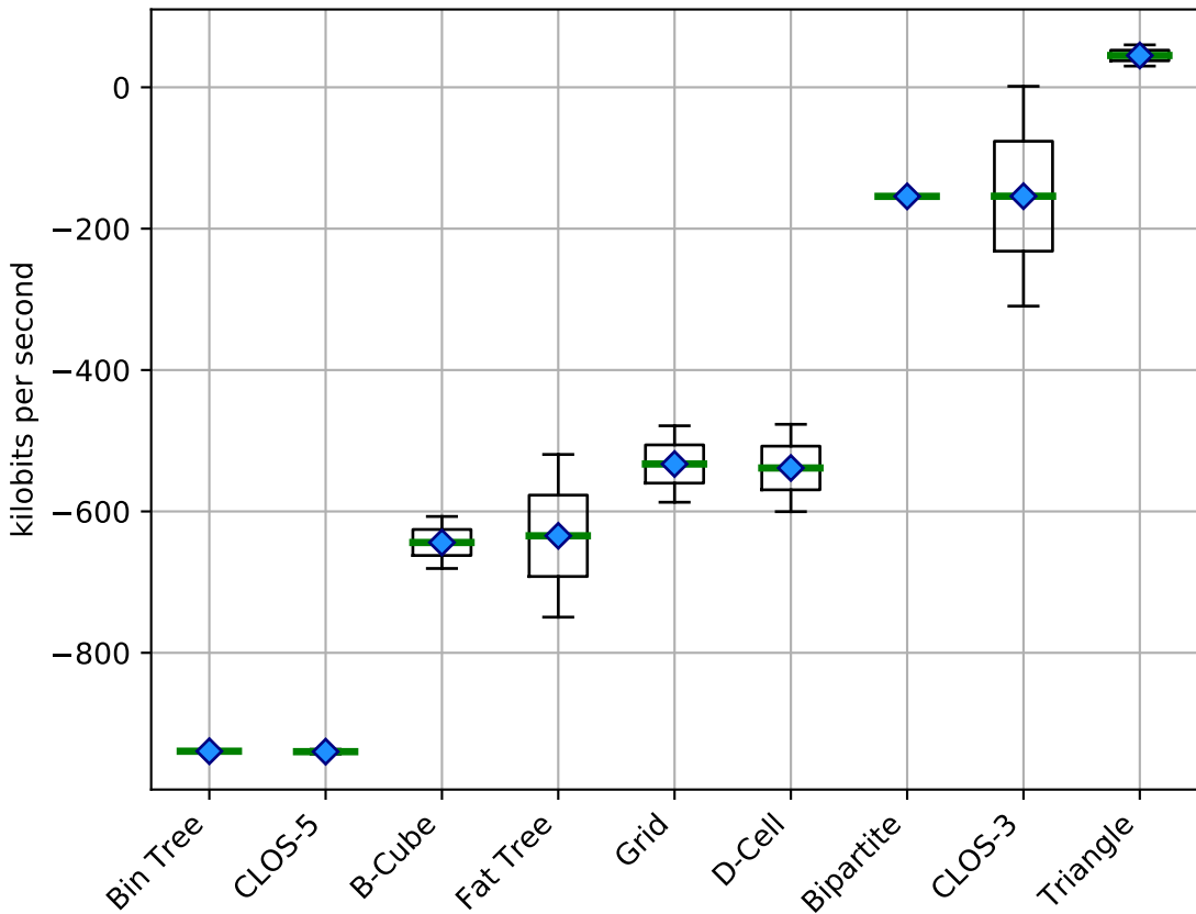
Bandwidth (impact) using LDR (multi-path)
