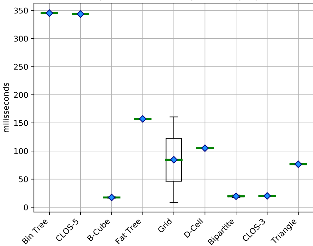
Latency (concurrent) using LDR (single-path)
