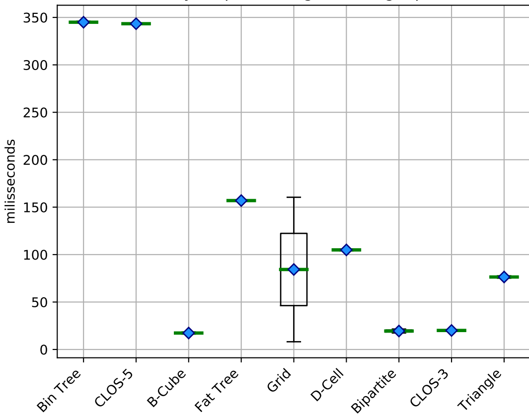
Latency (impact) using LDR (single-path)
