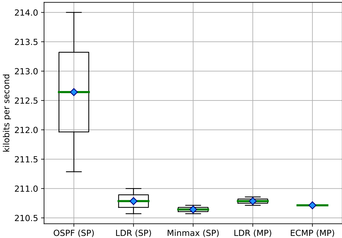
Bandwidth (concurrent) on Binary Tree
