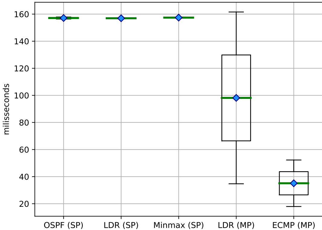
Latency (impact) on Fat Tree
