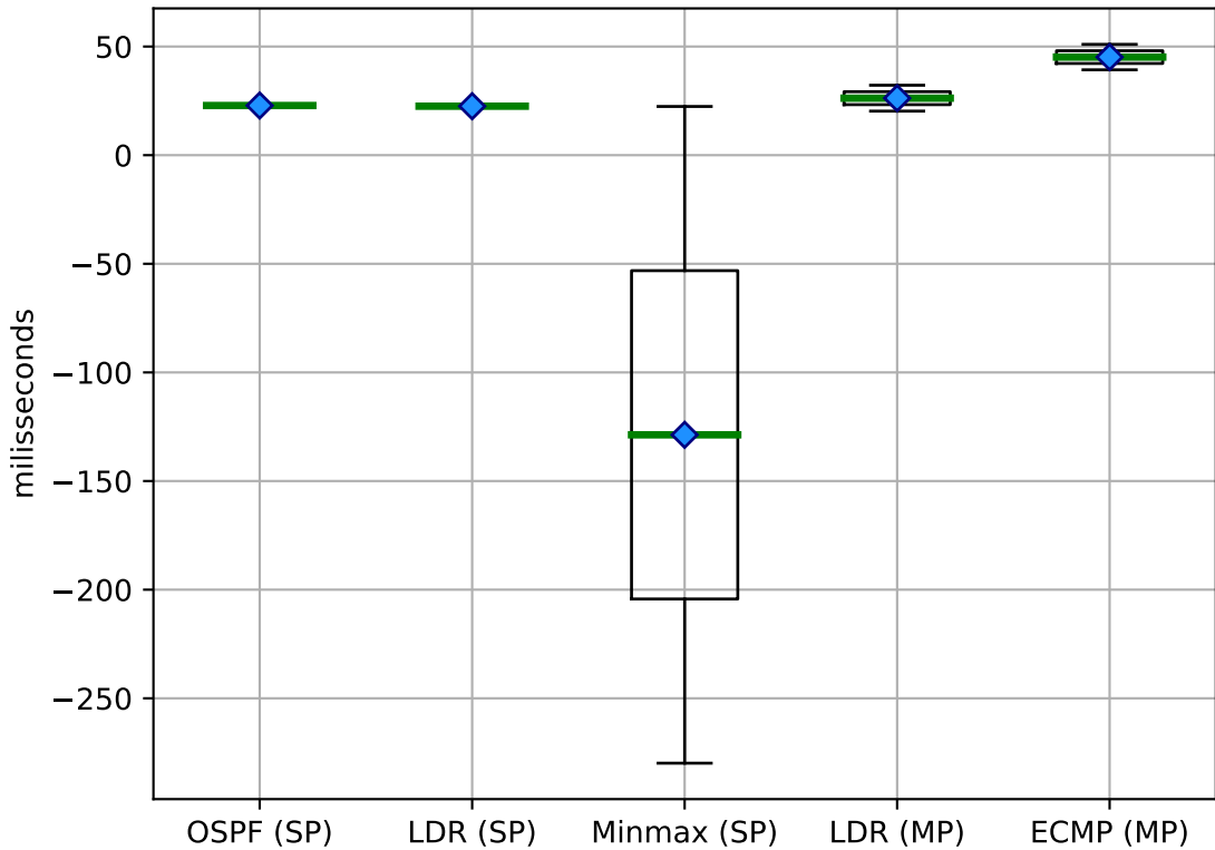
Jitter (impact) on D-Cell
