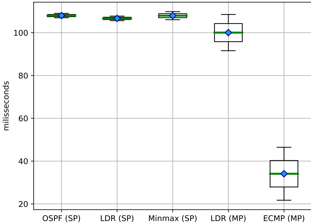
Jitter (impact) on 5-layered CLOS
