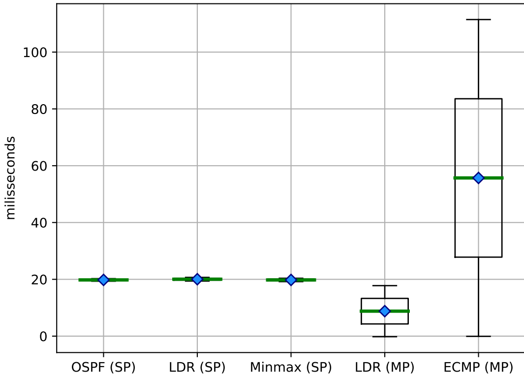
Latency (impact) on 3-layered CLOS
