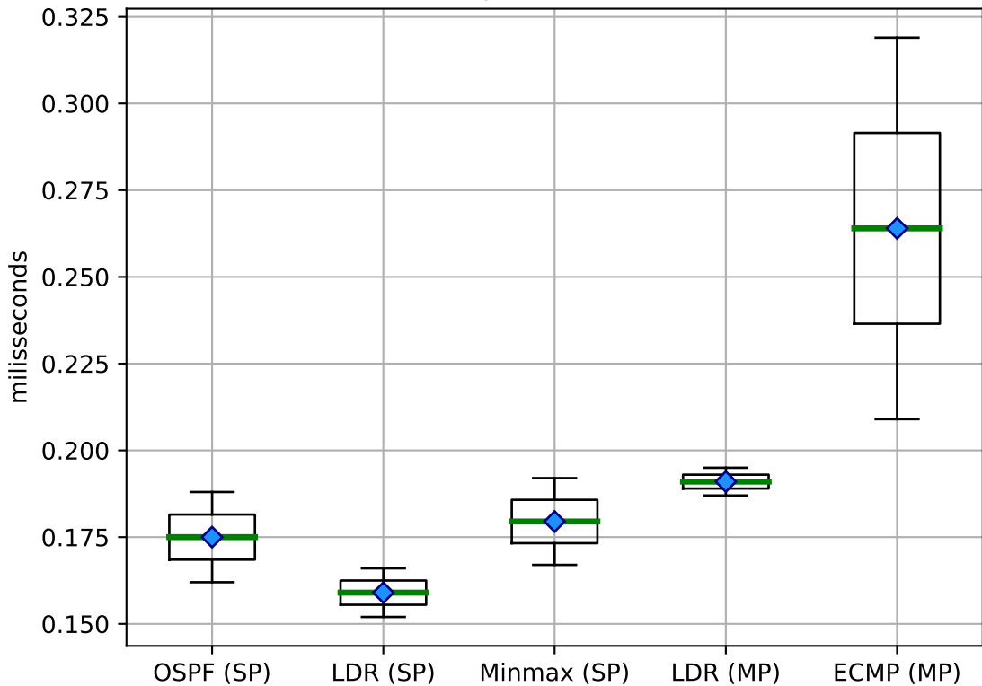
Jitter (sequential) on B-Cube
