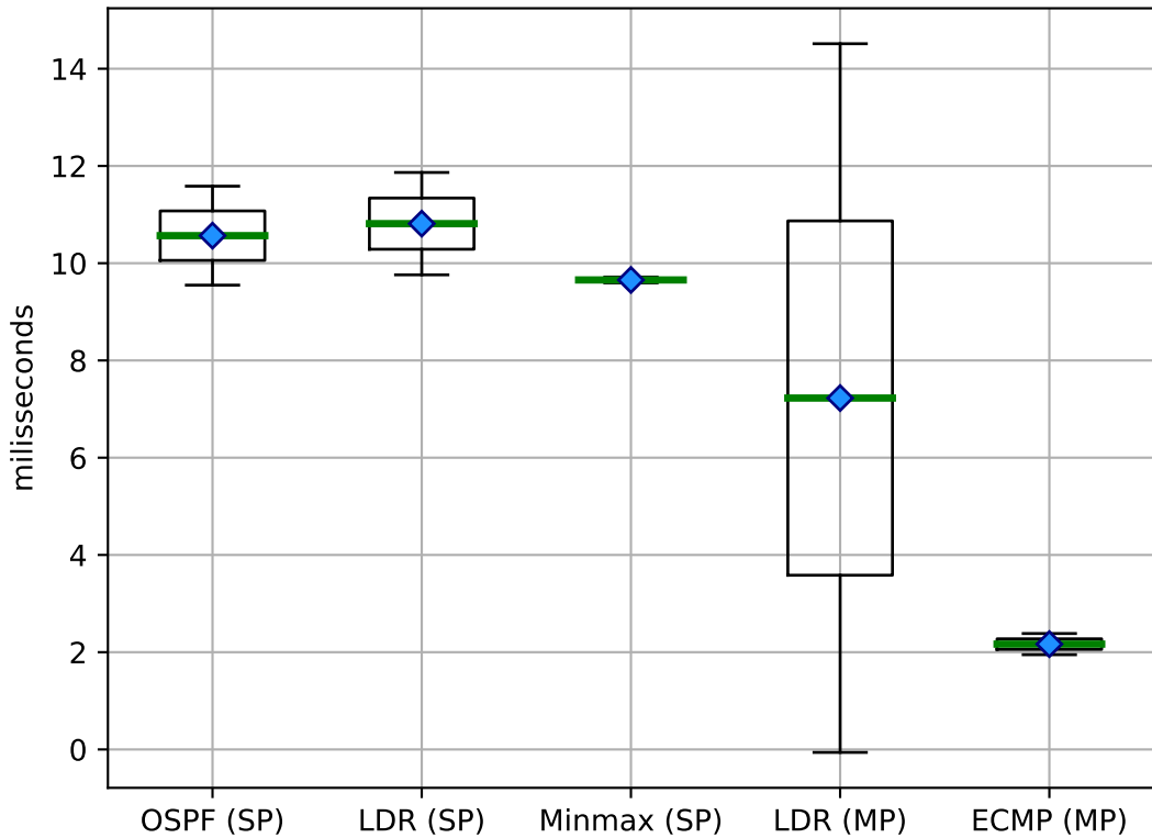
Jitter (impact) on B-Cube
