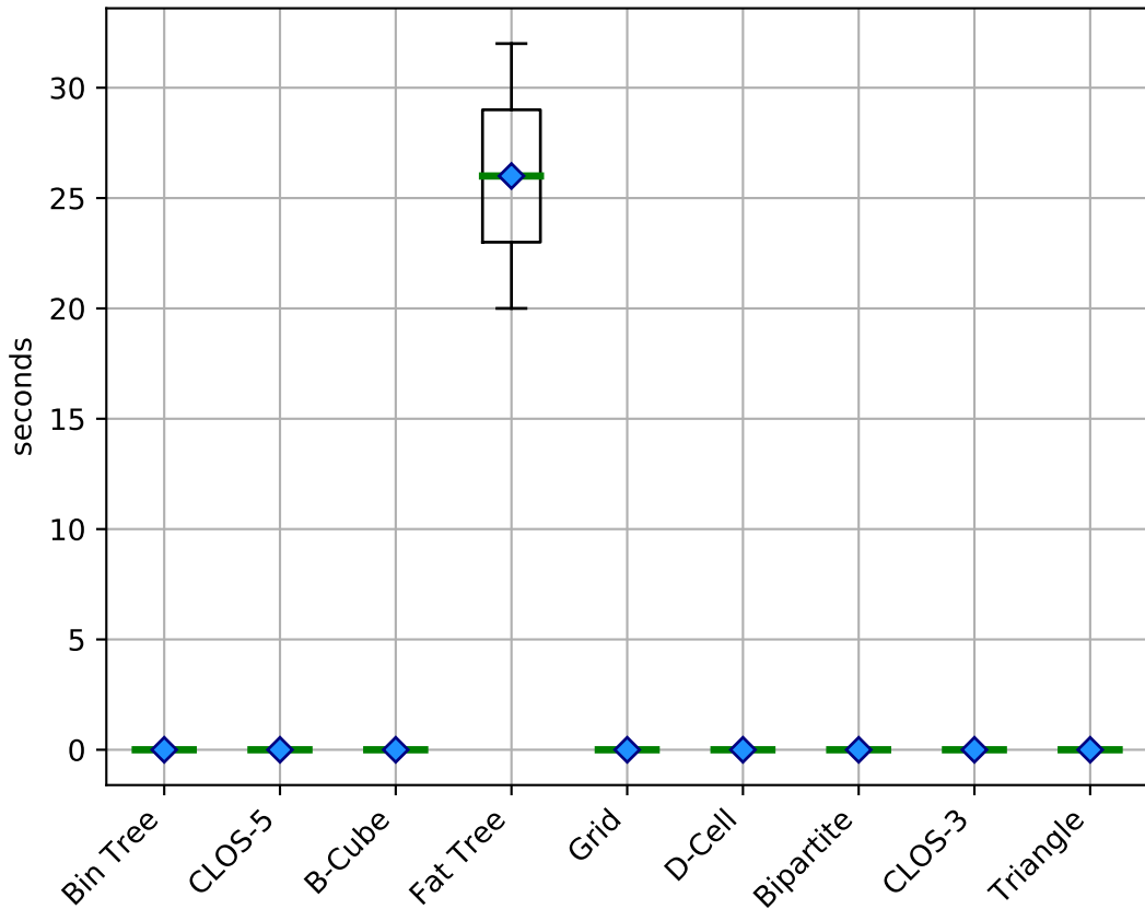
Routing response time using OSPF (single-path)
