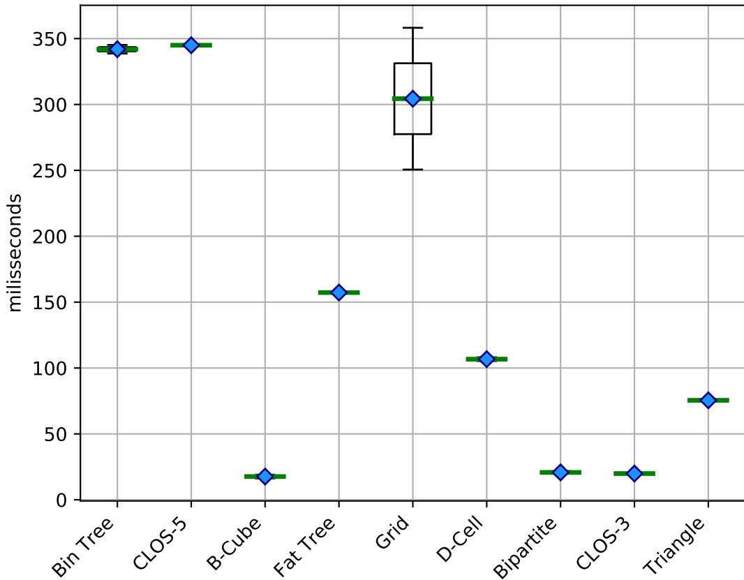
Latency (concurrent) using OSPF (single-path)
