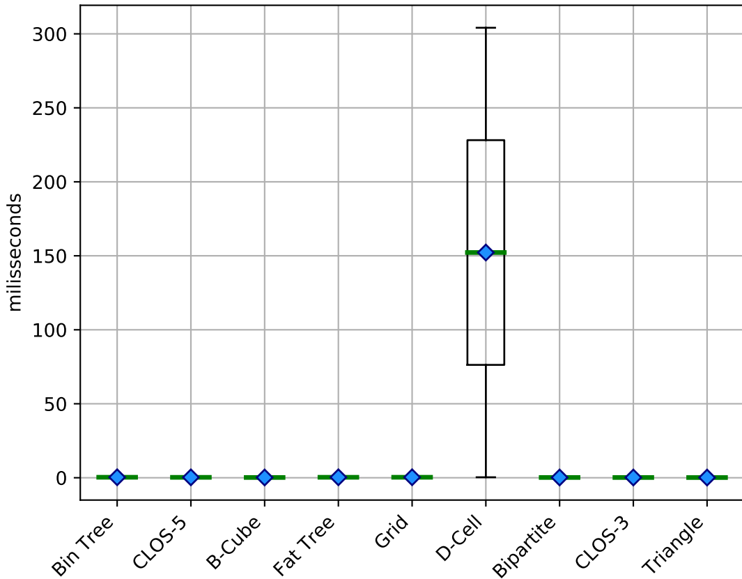
Jitter (sequential) using Minmax (single-path)
