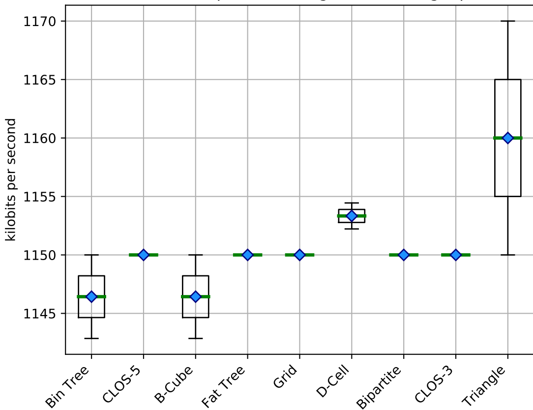
Bandwidth (sequential) using Minmax (single-path)
