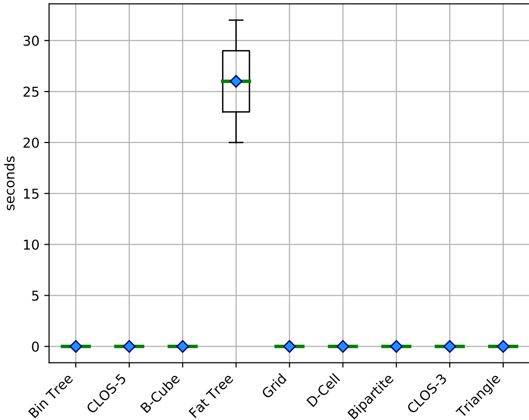
Routing response time using Minmax (single-path)
