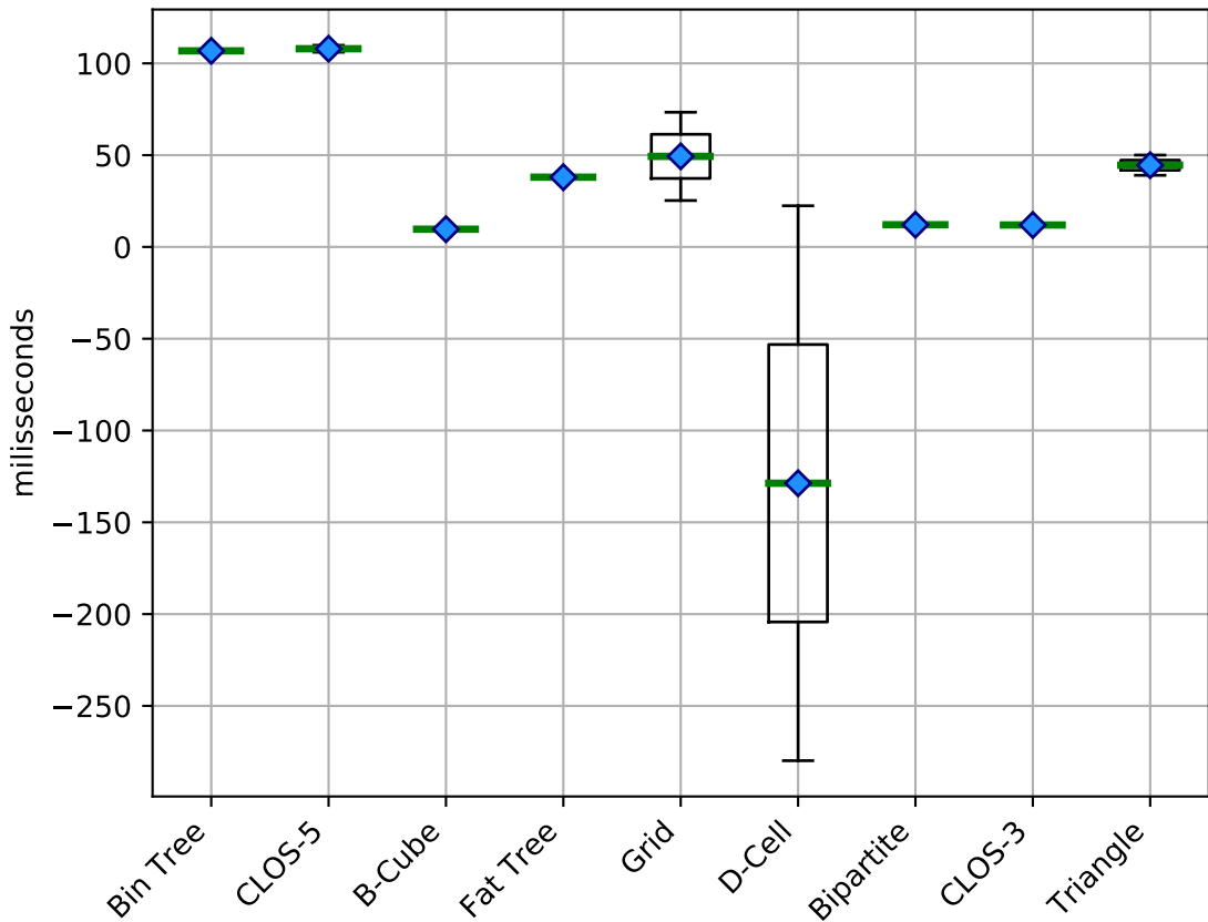
Jitter (impact) using Minmax (single-path)
