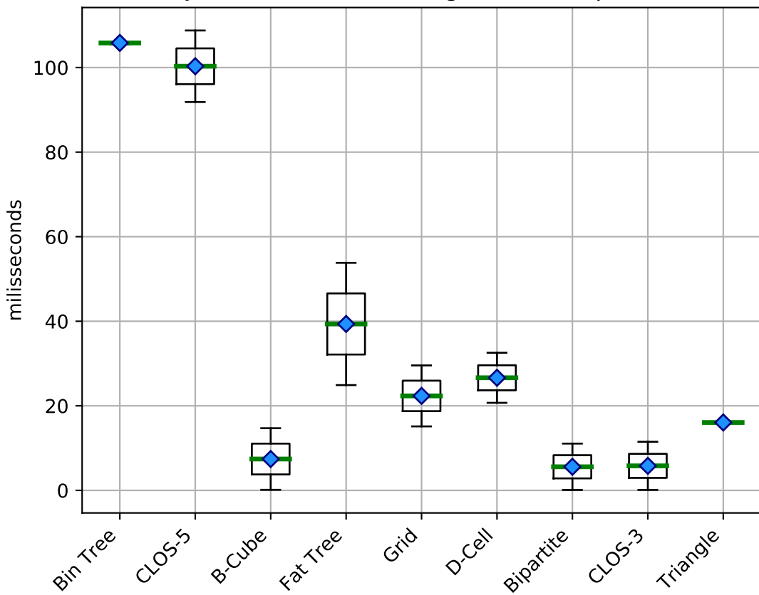
Jitter (concurrent) using LDR (multi-path)
