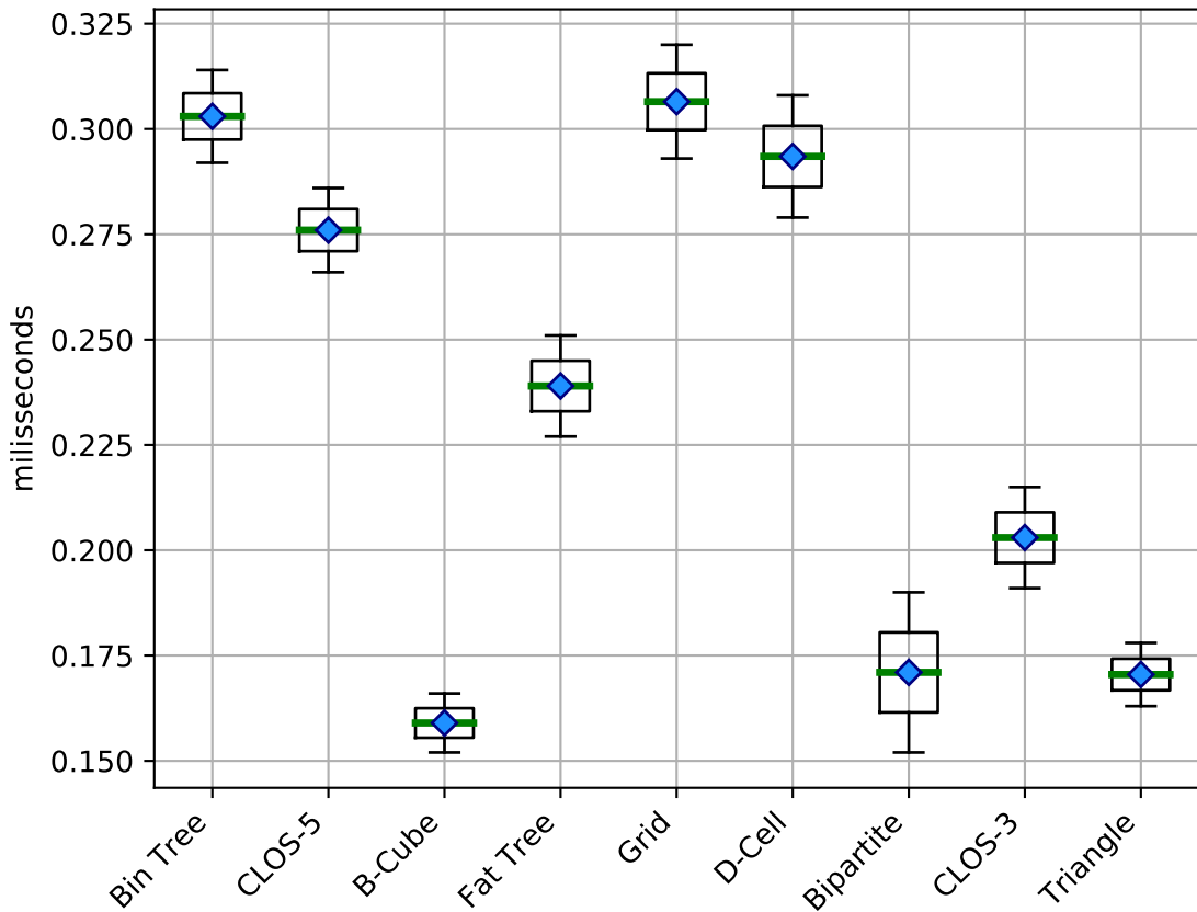
Jitter (sequential) using LDR (single-path)
