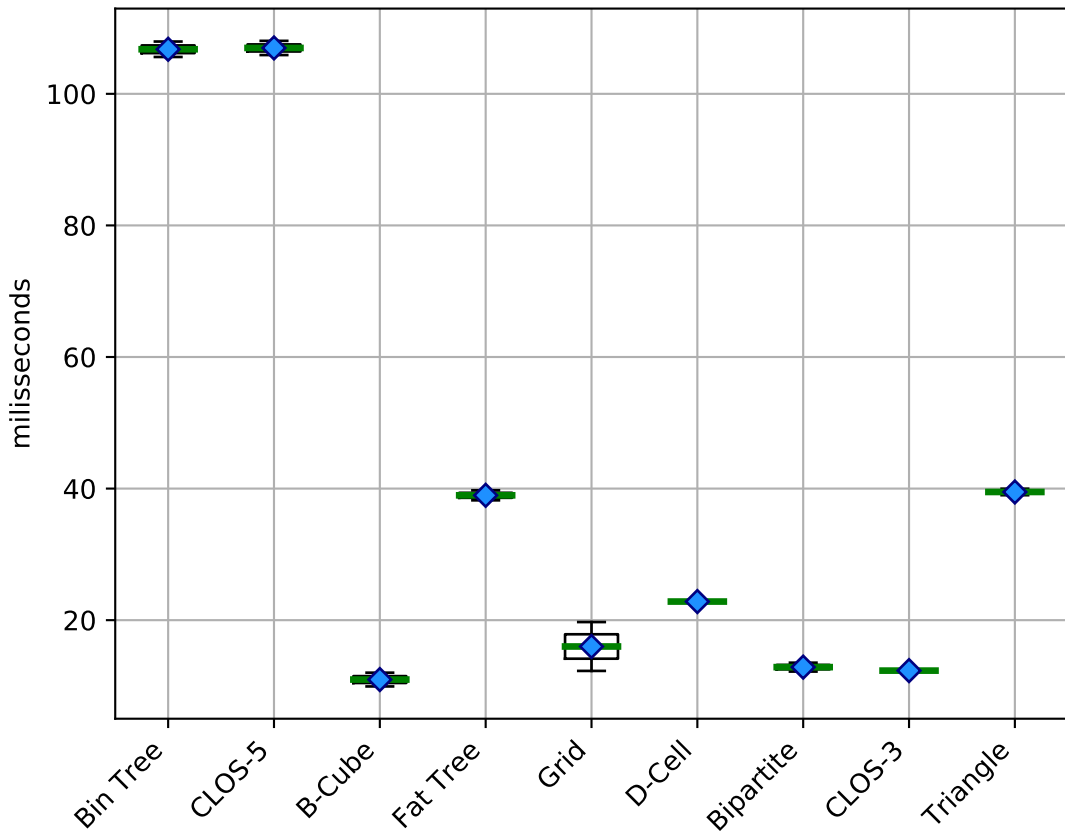
Jitter (concurrent) using LDR (single-path)
