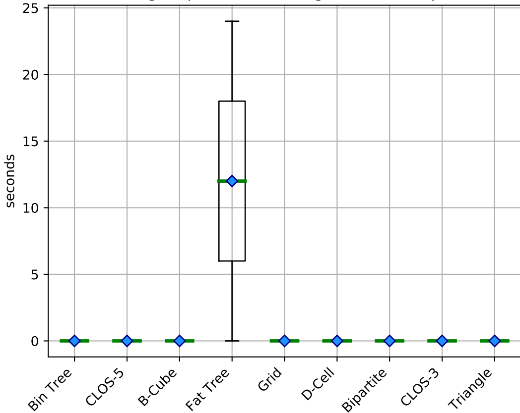
Routing response time using ECMP (multi-path)
