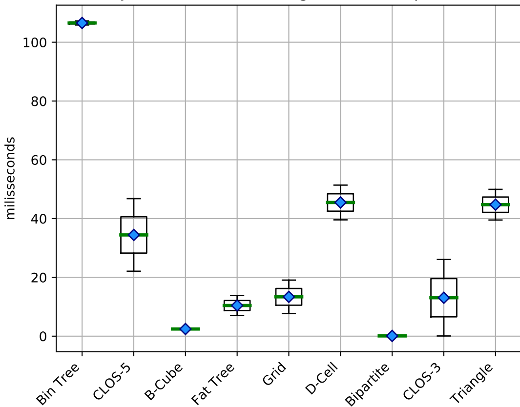
Jitter (concurrent) using ECMP (multi-path)
