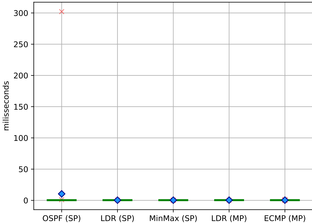
Jitter (sequential) on Binary Tree
