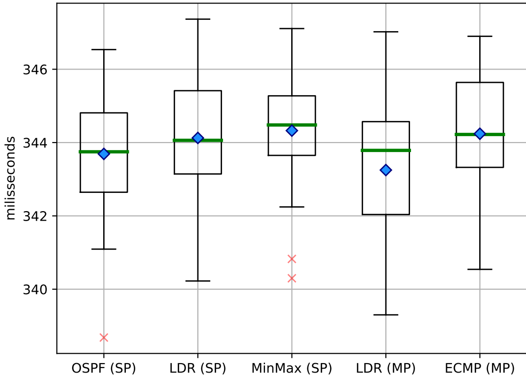
Latency (concurrent) on Binary Tree
