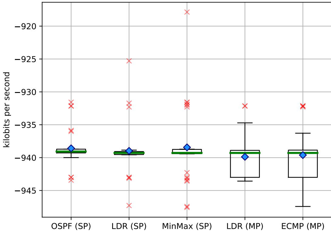
Bandwidth (impact) on Binary Tree
