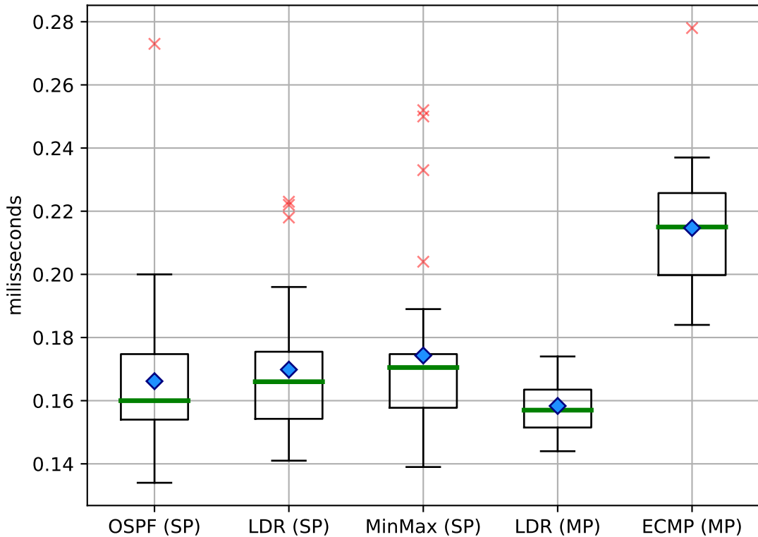
Latency (sequential) on Fat Tree
