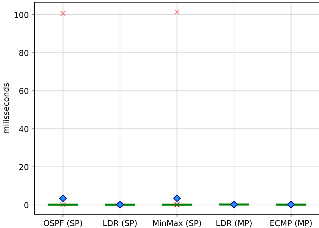
Latency (sequential) on D-Cell
