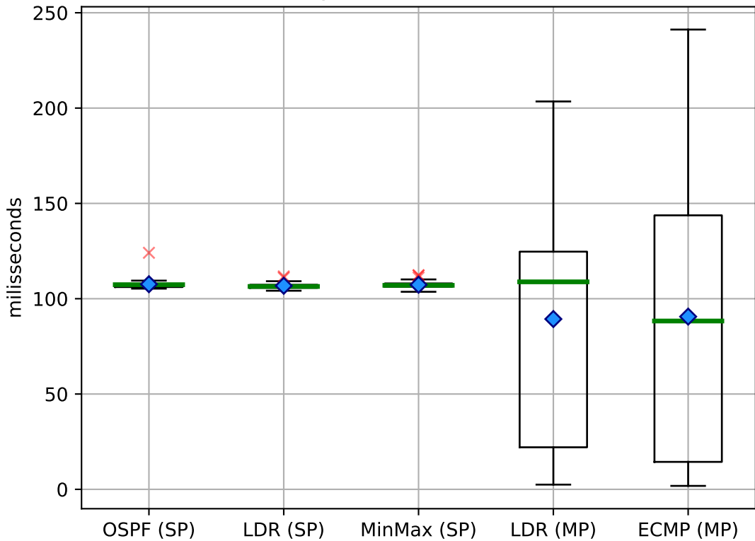
Latency (concurrent) on D-Cell
