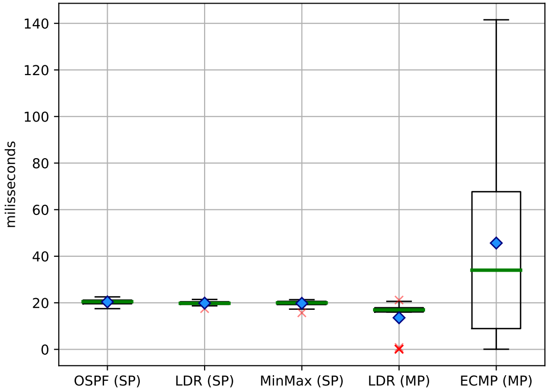
Latency (concurrent) on 3-layered CLOS
