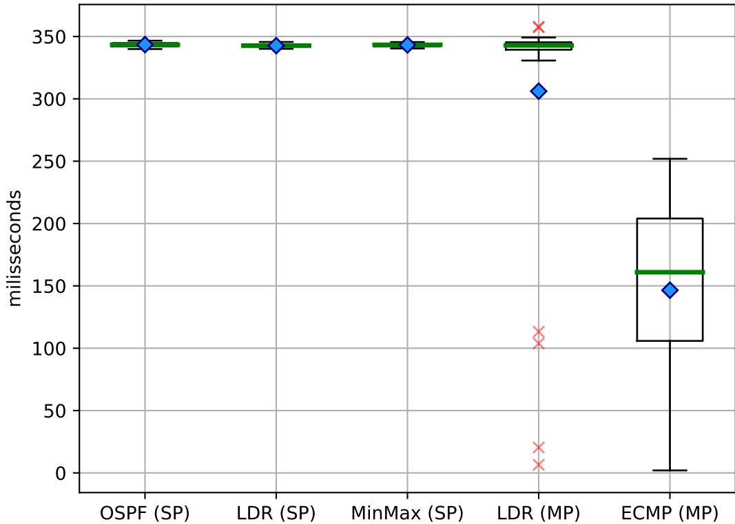
Latency (impact) on 5-layered CLOS
