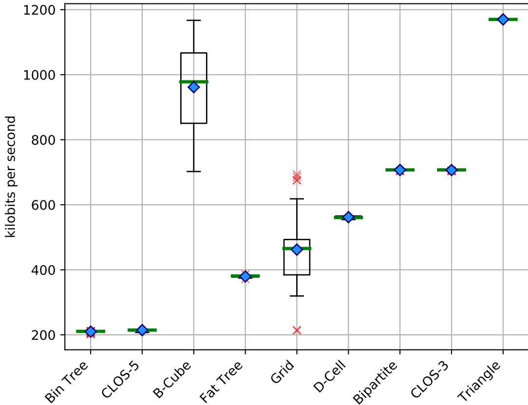
Bandwidth (concurrent) using MinMax (single-path)
