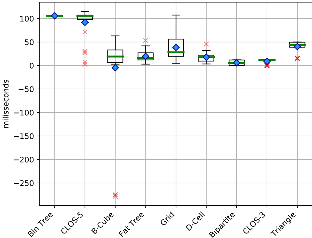
Jitter (impact) using LDR (multi-path)
